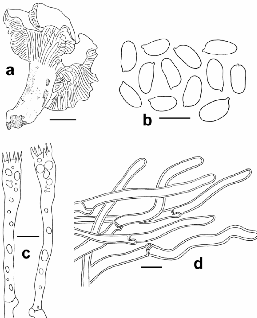
Fig. 1. C. ilicis (holotype). a) Silhouette of a basidiome ( Bar = 10 mm). b) Basidiospores. c) Basidia. d) Pileipellis hyphae. (1b, 1c and 1d, Bar = 10 mm).
